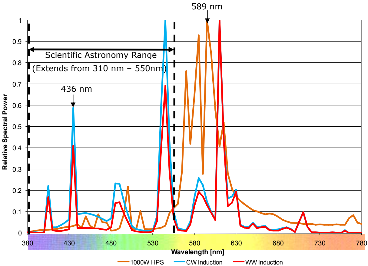
Figure 25: Spectral Power Distribution Curves Comparing HPS and Induction Sources.
