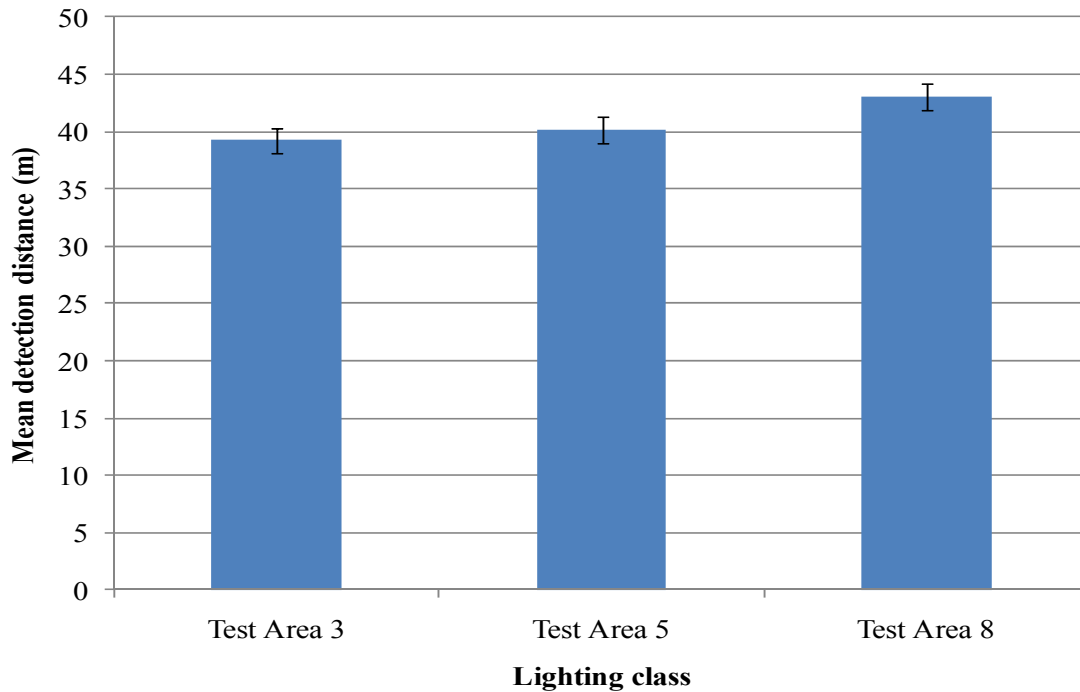
Figure 20: Pedestrian (Hardhat) Performance for Intersection Test Areas
